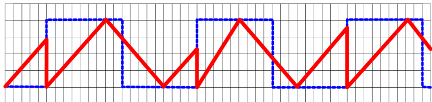
Triangle Wave Hard Sync'd to Pulse Wave
